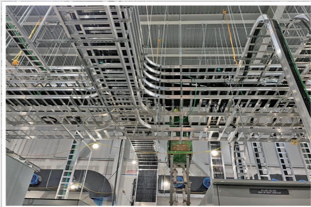
Cable Tray Installation
