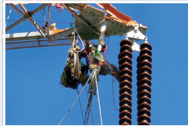
Insulator Installation
